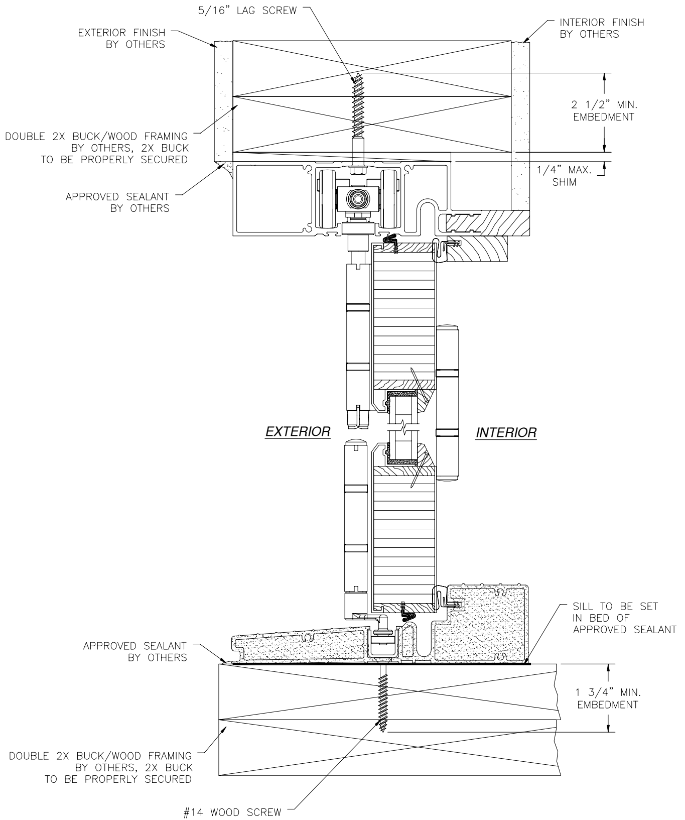
VERTICAL CROSS SECTION 2X BUCK/WOOD FRAMING
