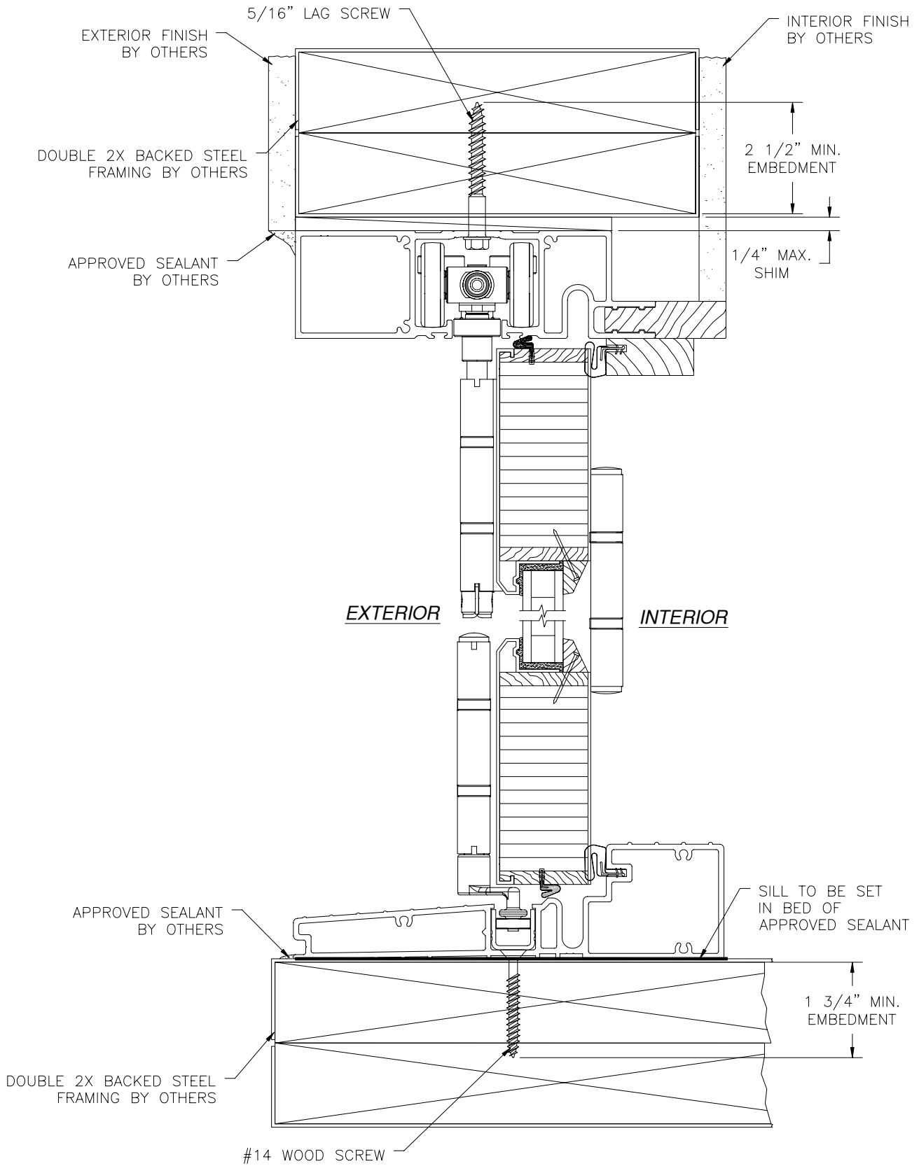
VERTICAL CROSS SECTION DOUBLE 2X BACKED STEEL FRAMING
