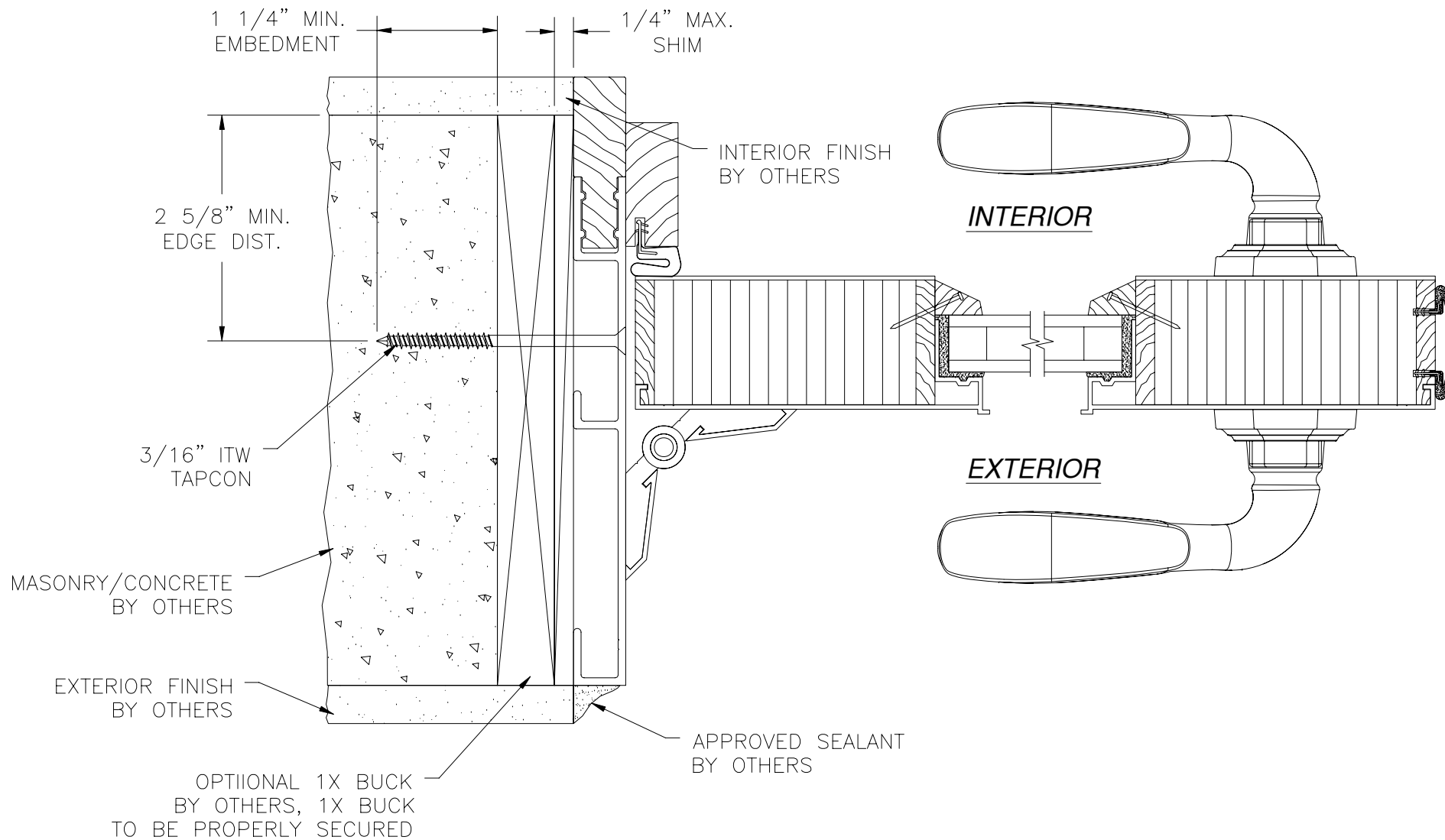
HORIZONTAL CROSS SECTION MASONRY/CONCRETE INSTALLATION
